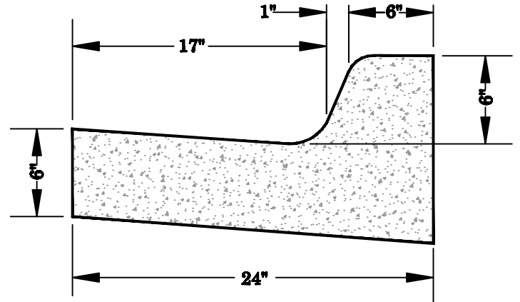
VERTICAL CURB
